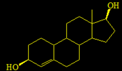
19-Nor-4-androstenediol
