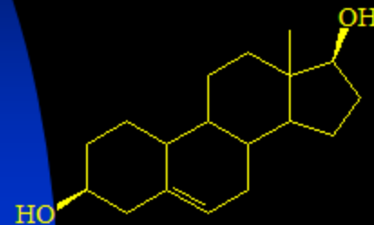
19-Nor-5-androstenediol
